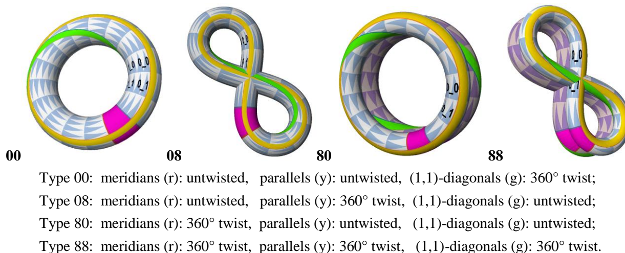
Figure 2: Tori in four different homotopy classes and their characterization by the amount of twisting of some characteristic ribbons embedded in their surfaces.
