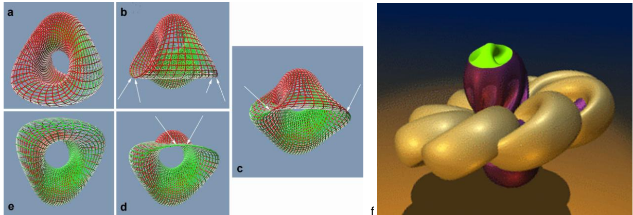
Figure 13: Parameter swap: (a \rightarrow e) Conceptual – using non-immersive intermediate steps. (f) A valid but cumbersome approach making use of the classical “Outside-In” sphere eversion process [6].
